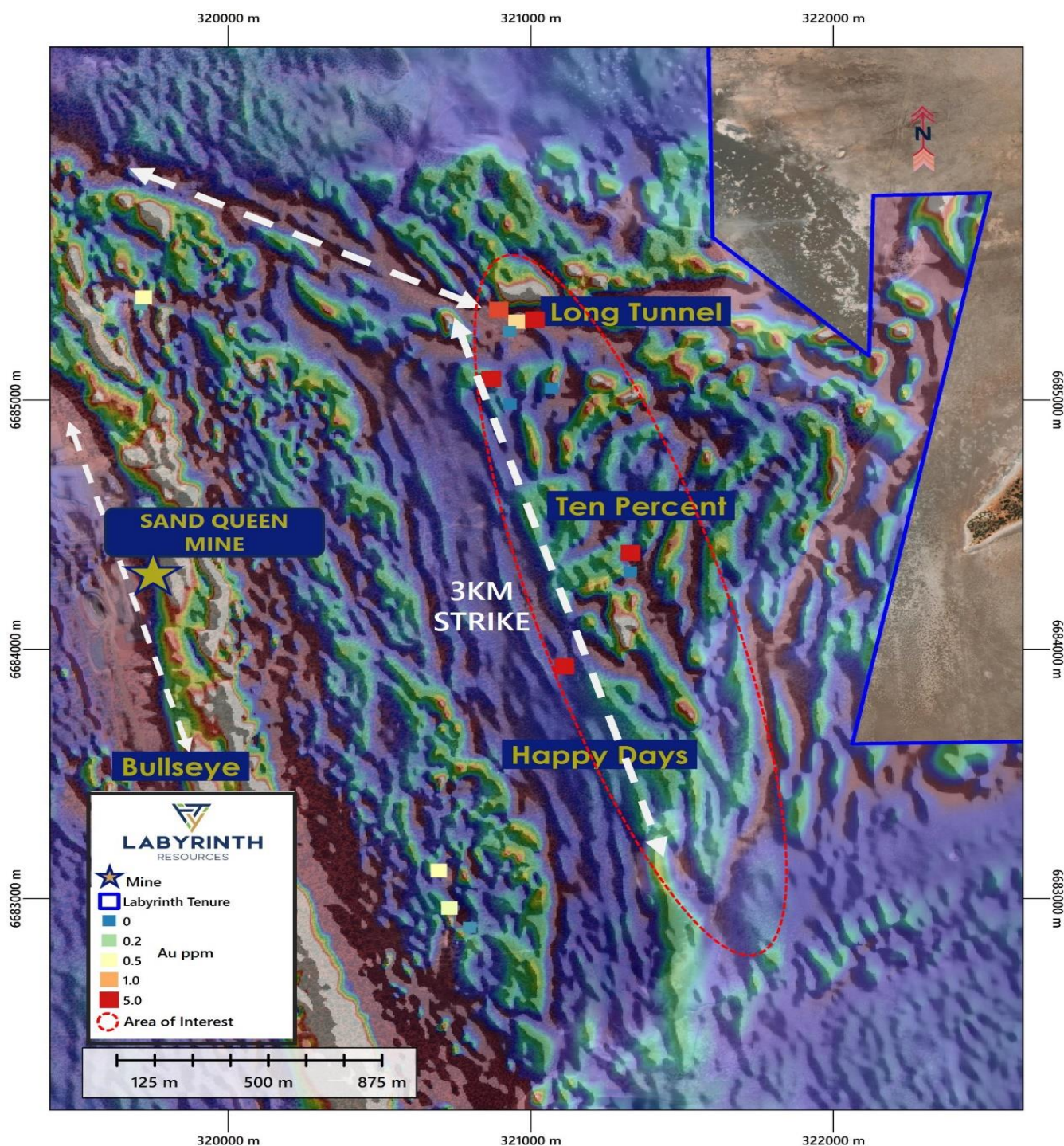
Figure 2. TMI1VD with NE shading overlain with TMI2VD shows structures and apparent folding. Mineralisation occurs in contact with s 3km long NNW-SSE shear zone.
