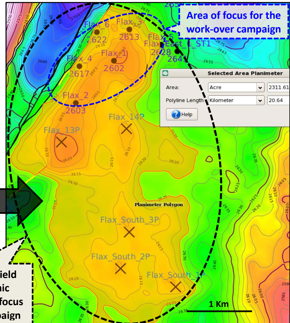
New Top Tirrawarra Depth Map – 3D Seismic - 2012
