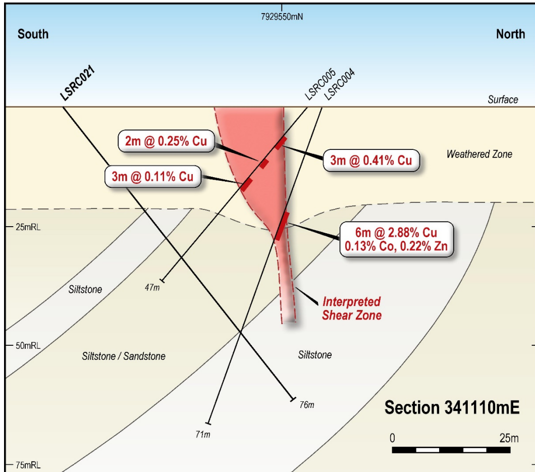
Figure 4: Cross section view of drilling at Lincoln Springs prospect. Section 341110mE.
