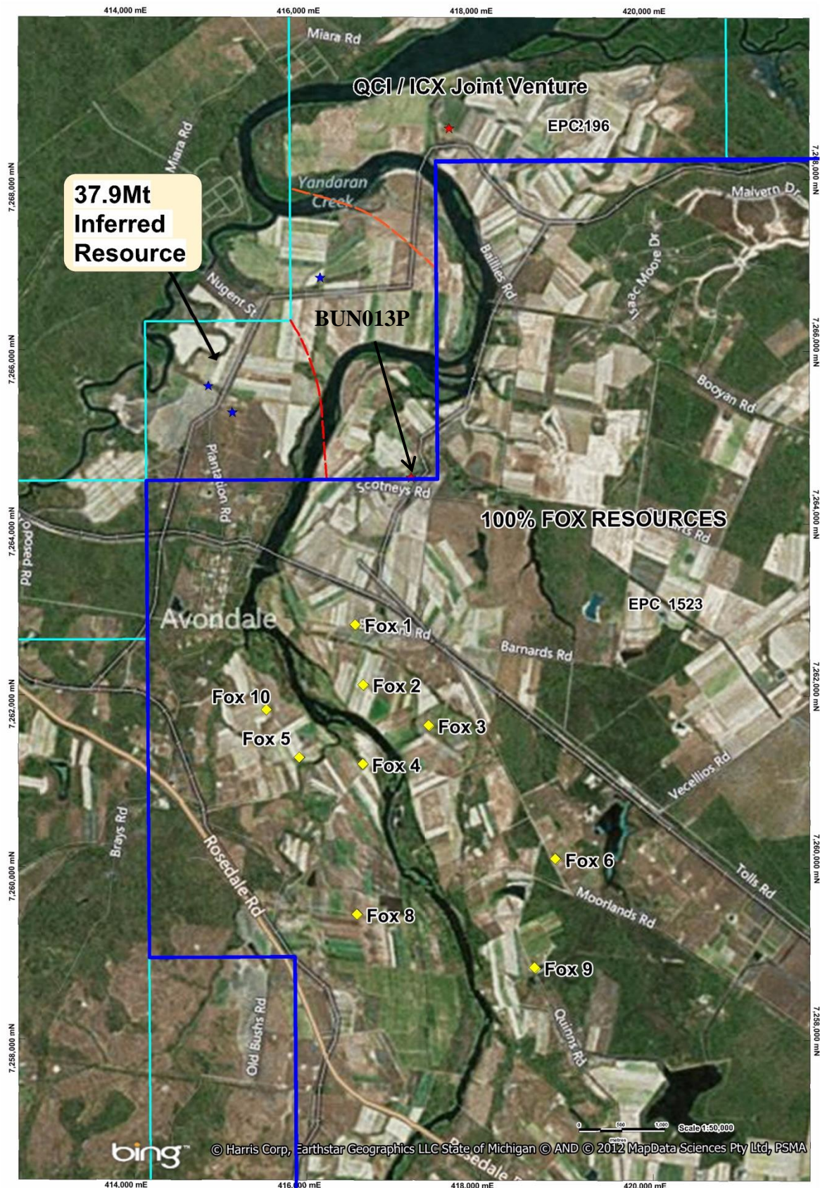
Figure 1: Fox Resources drilling at the Bundaberg Coking Coal project
