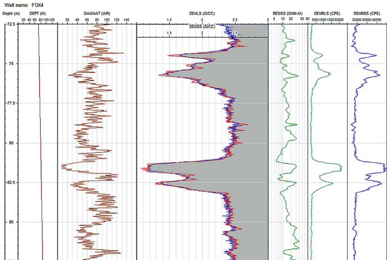
Figure 2: Fox 4 Geophysical logging from 72.5m to 87.5m down hole. Logging occurred through the drill rods.
